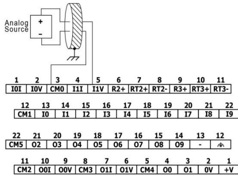
Differential
