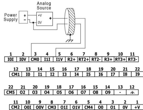
Single-ended
