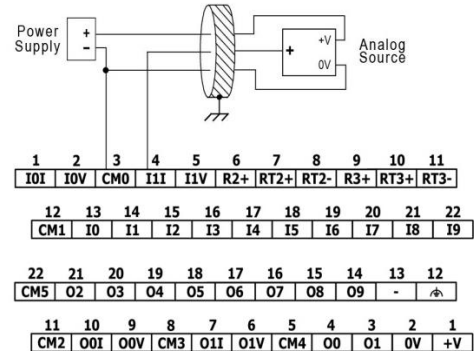
3-wire
