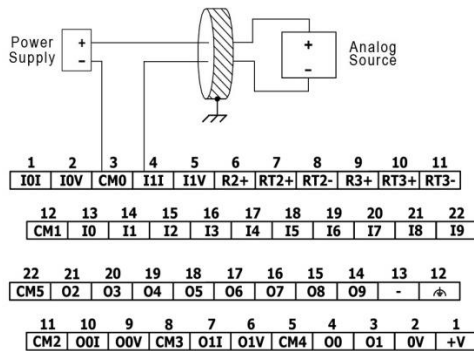
2-wire
