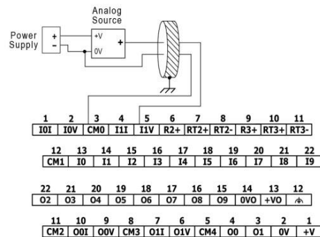
Single-ended
