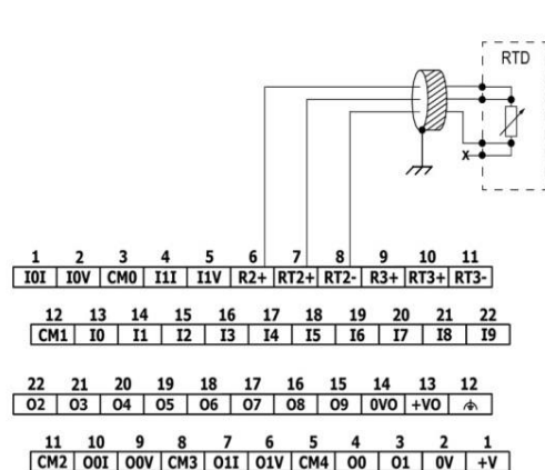
4-wire
