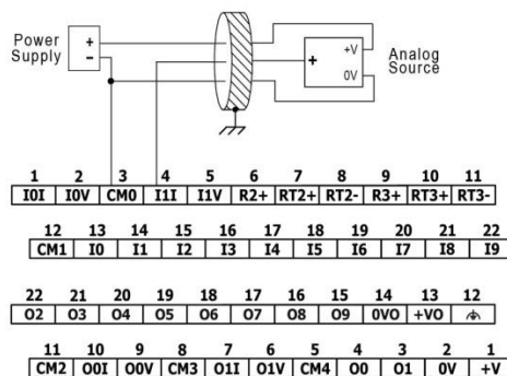
3-wire
