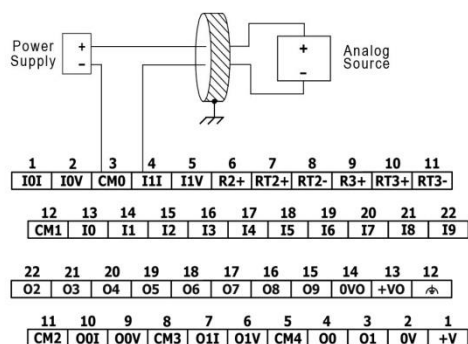
2-wire
